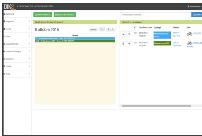
schermata HOME
